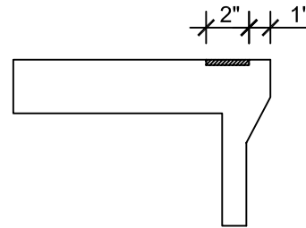
CLASSIC PROFILE WITH INTEGRAL AGGREGATE WARNING DETAIL
