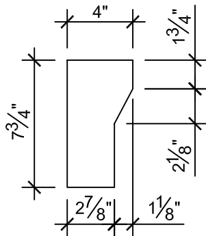
CLASSIC PROFILE STARTER STEP
